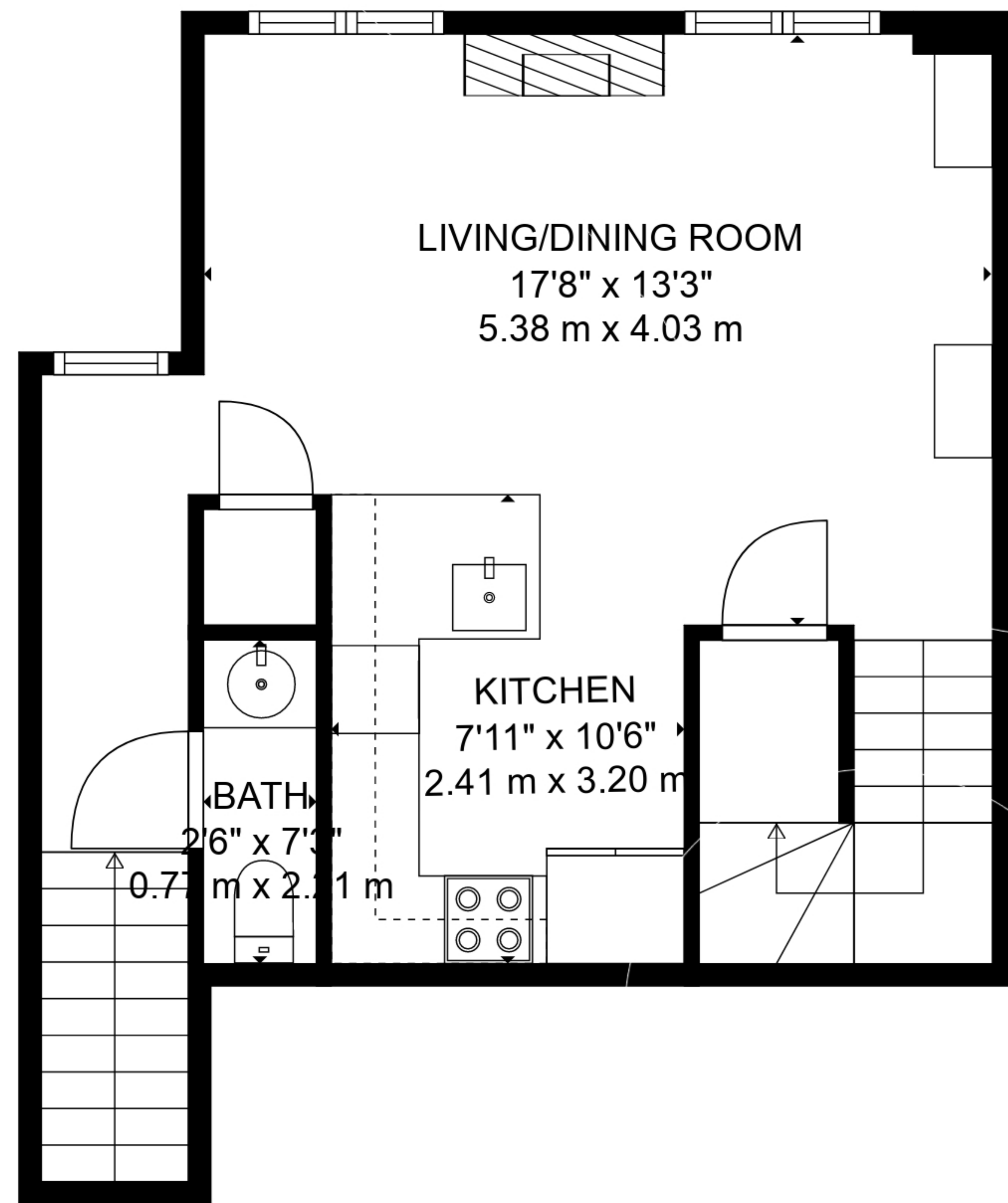
FLOOR 1
