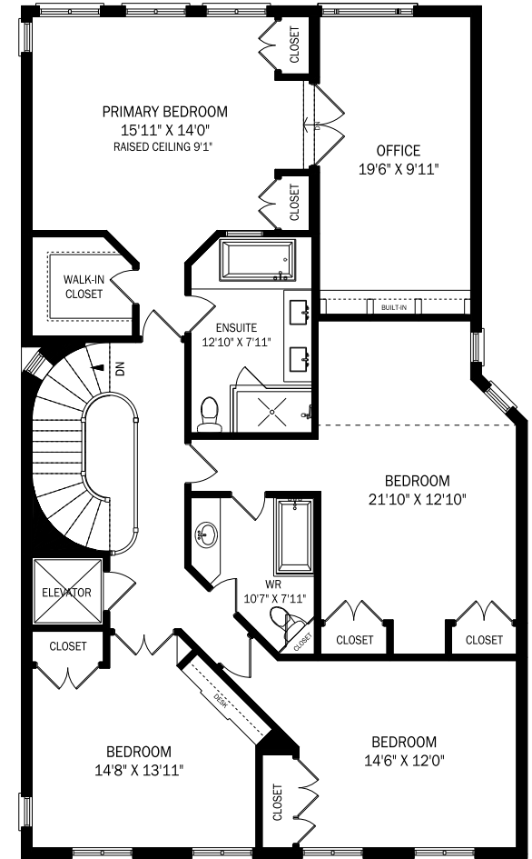
CEILING HEIGHT 8'3" SECOND FLOOR - 1775 SQUARE FEET
