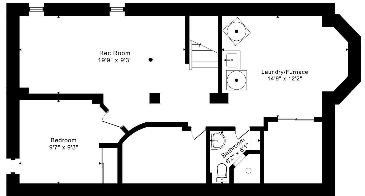
LOWER FLOOR 895 SQUARE FEET
