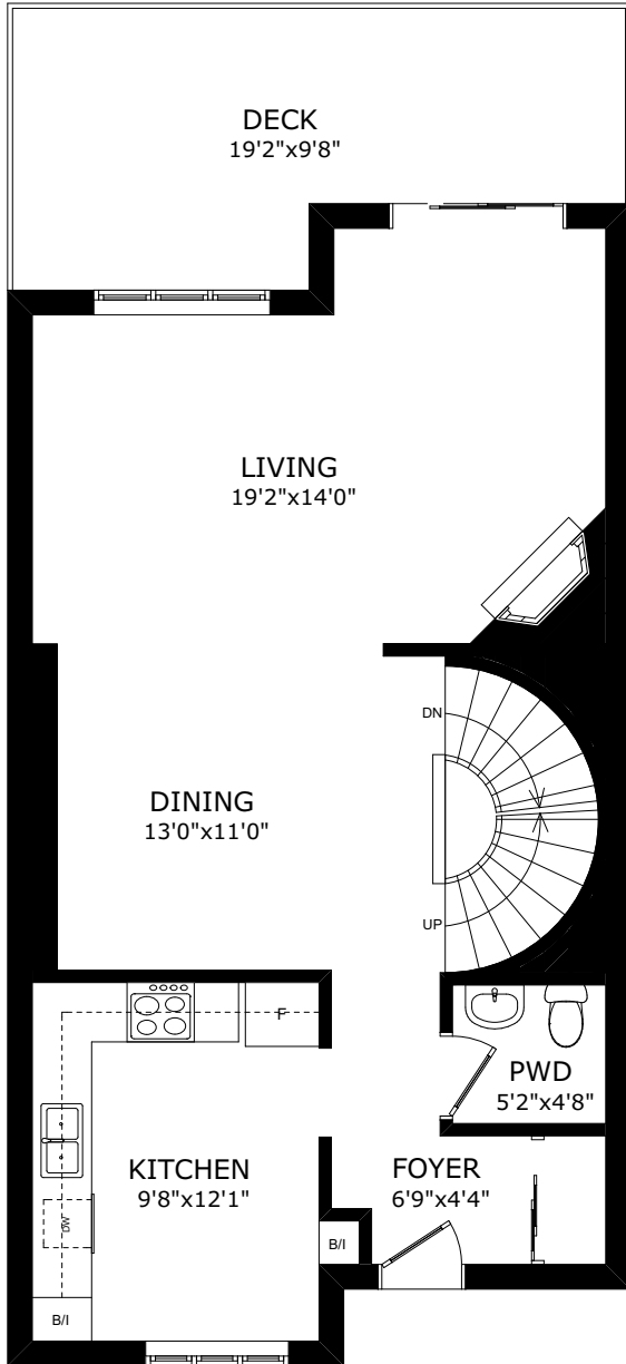
MAIN FLOOR
