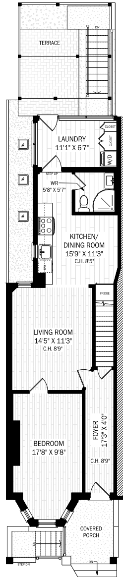
MAIN FLOOR - 782 SQUARE FEET
